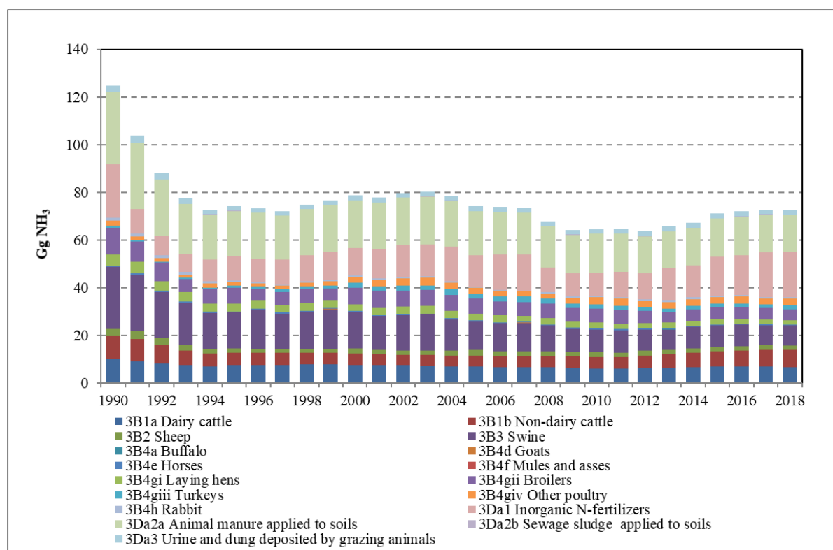
Figure 5.2. Emissions of NH 3 , 1990-2018
